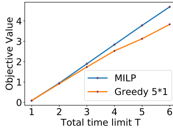
Fig. 7. Expected threat value patrolled with different total time limit.
