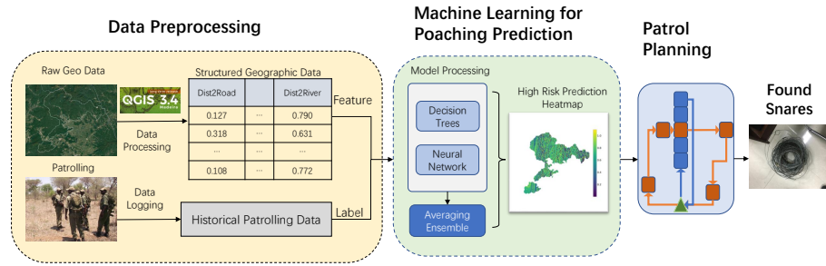
Fig. 1. The workflow of this study. The images in this figure are just for example and not our result.
