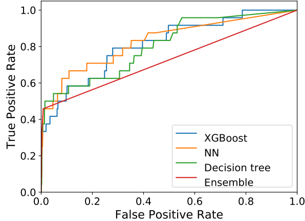
Fig. 4. The ROC Curve of our models.
